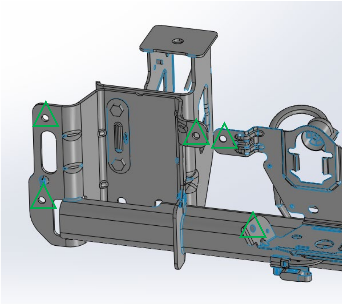
Figure 3c (5x Bolt Locations per Side)
